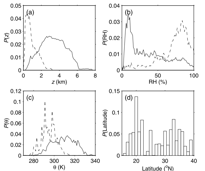
Figure 2. Probability distribution functions of the number of data points with respect to (a) altitude, (b) relative humidity, (c) potential temperature, and (d) latitude. For (a) through (c) the solid line represents the free troposphere and the dashed line denotes the boundary layer.
